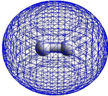
MO \sigma
