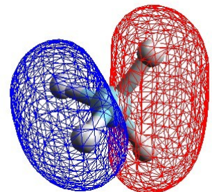
MO \sigma_4
