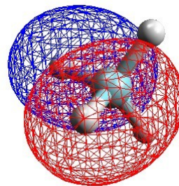
MO \sigma_3
