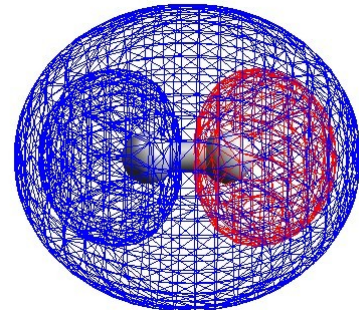
MO \sigma + MO \sigma^*
