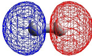
MO \sigma^*
